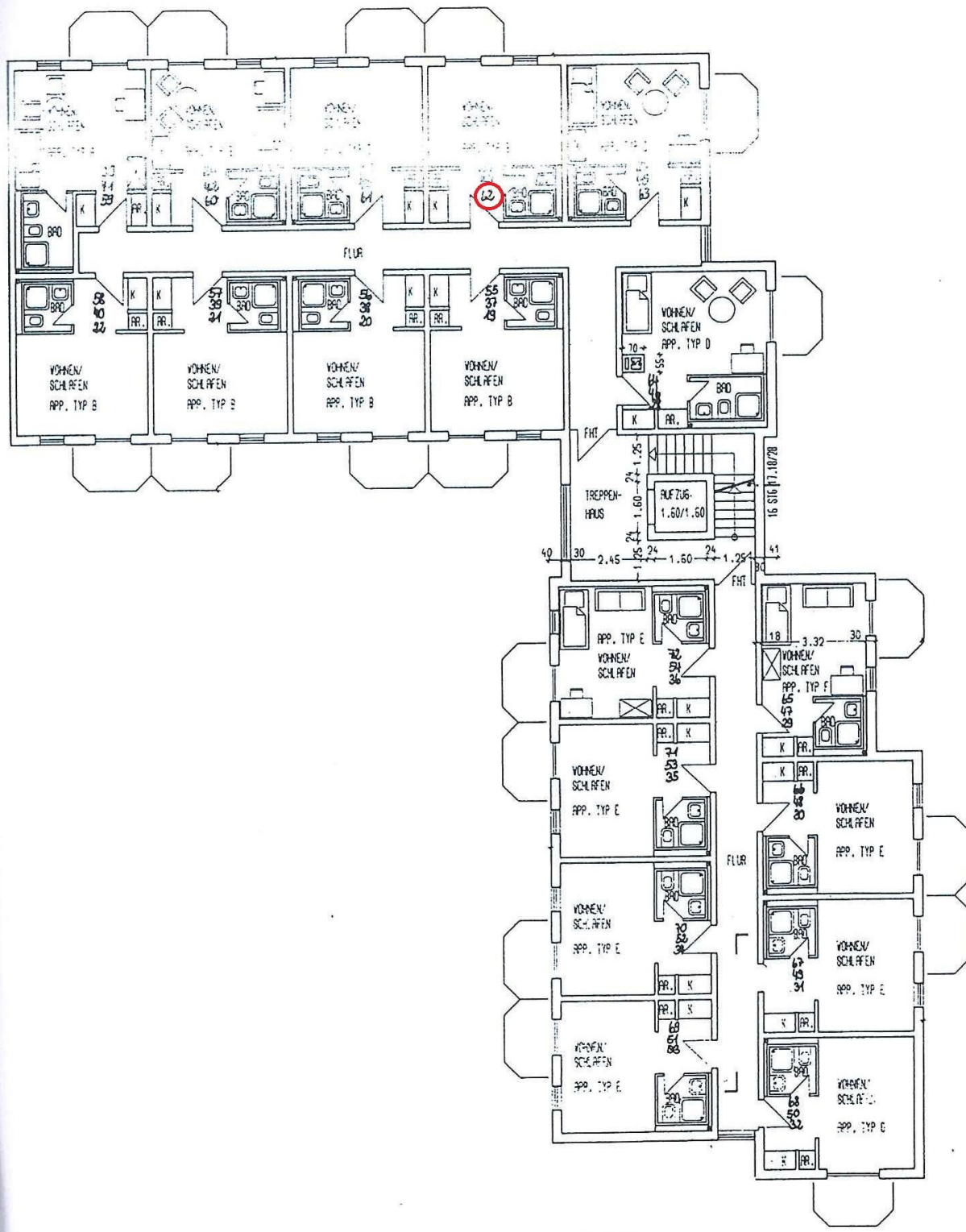
Grundriss Apartment
